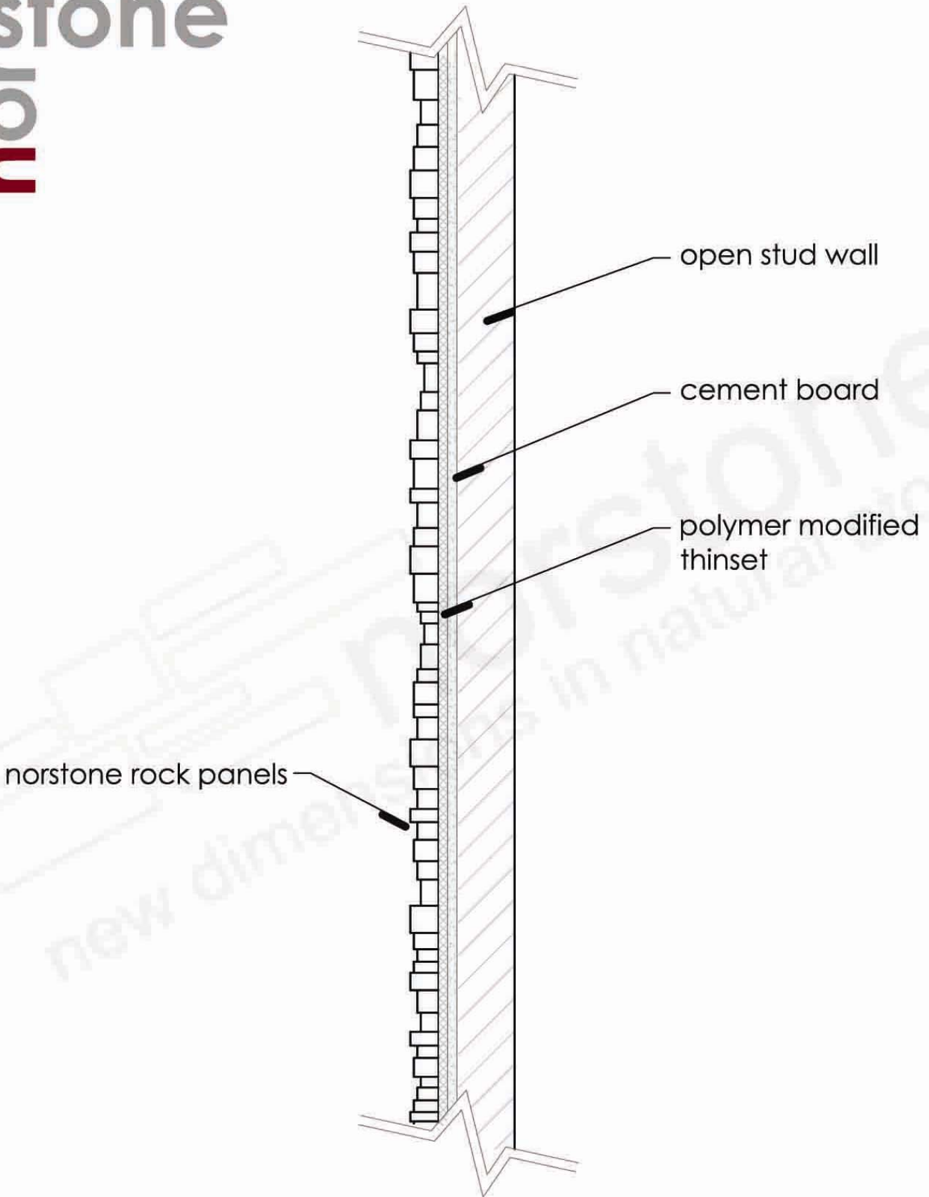
rock panel detail - open stud wall - interior
